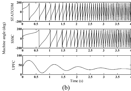
Fig. 6. Swing curve of the machine for various operations of UPFC: (a) Fault clearing time= 235ms; (b) Fault clearing time= 245ms
