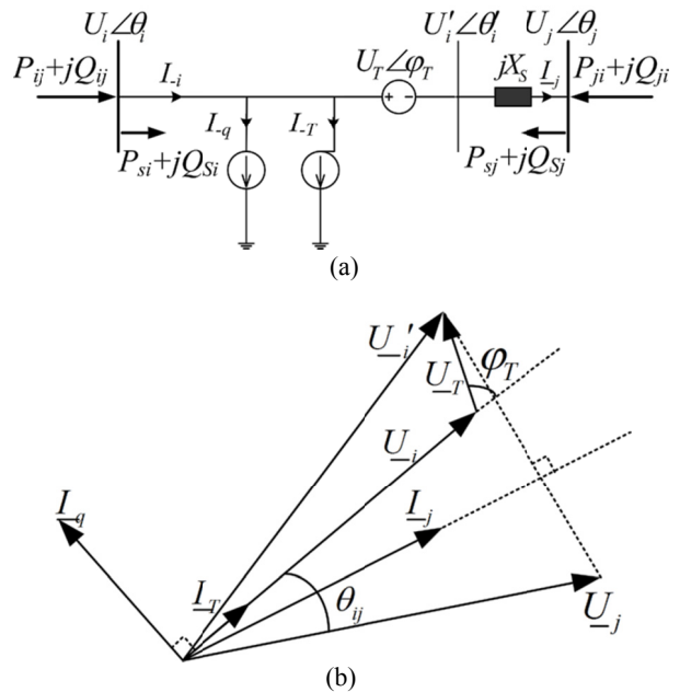
Fig. 2. (a) Basic model of the UPFC and the injected powers; (b) Phasor diagram
