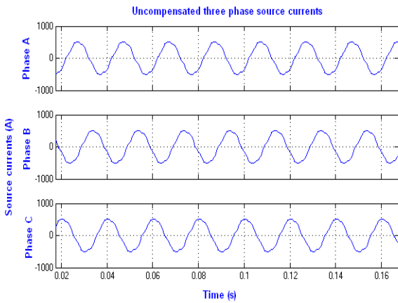
Fig. 4. Three phase source currents for uncompensated DSTATCOM in PS.
