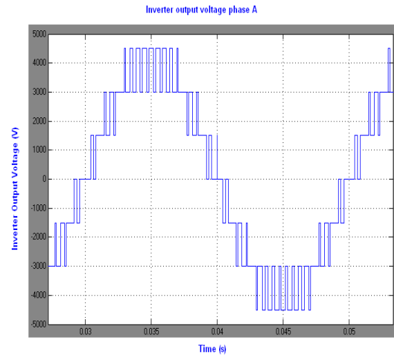
Fig. 11. Inverter output voltage for phase - a.
