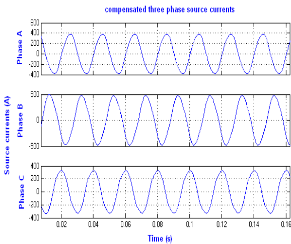
Fig. 6. Three phase source currents for compensated DSTATCOM in PS.
