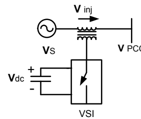
Fig. 1. Structure and type of connection to DVR network
