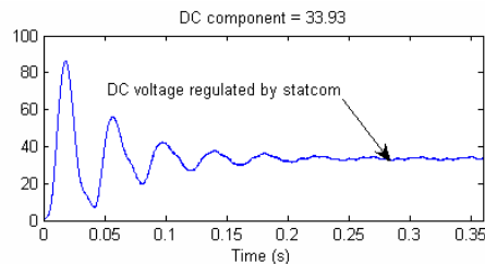
Fig. 16. Adjusted DC link voltage by STATCOM
