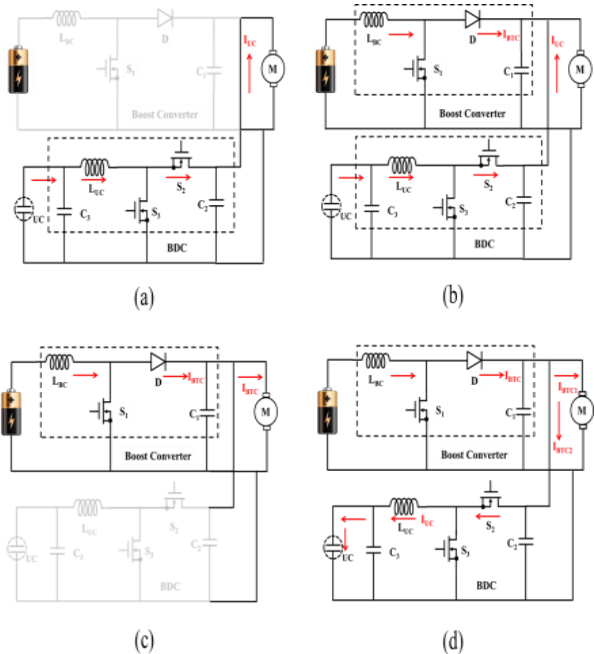
Fig. 8. (a).Converter model1 circuit diagram with HESS, (b).Converter mode2 circuit diagram with HESS, (c).Converter mode3 circuit diagram with HESS, (d).Converter mode 4 circuit diagram with HESS.
