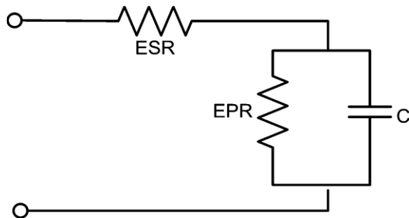
Fig. 3. Equivalent electrical model of UC.
