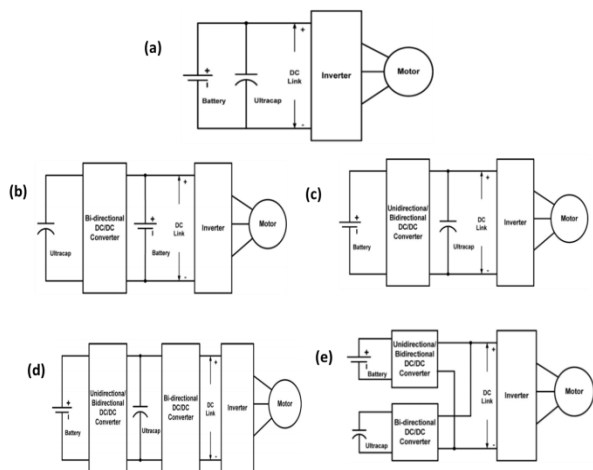
Fig. 1. (a) Conventional paralleling of sources, (b) UC-Battery model, (c) Battery-UC model, (d) Cascaded model, (e) Multiple Converter models.
