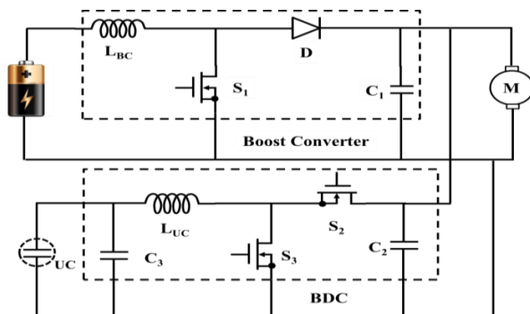
Fig. 7. Converter main circuit diagram with HESS.
