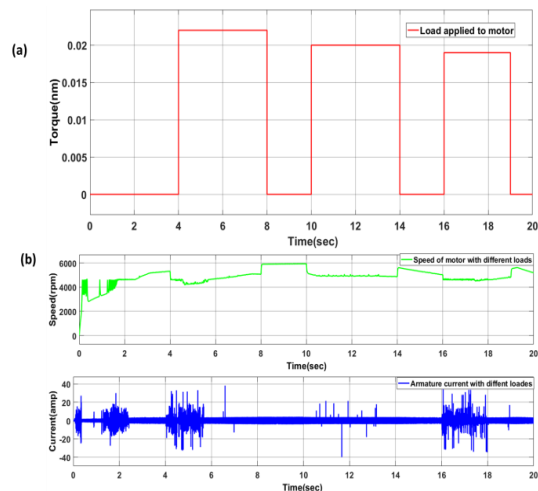
Fig. 10. (a). The load applied to the motor. (b) Speed and current curve variations with respect to the load.
