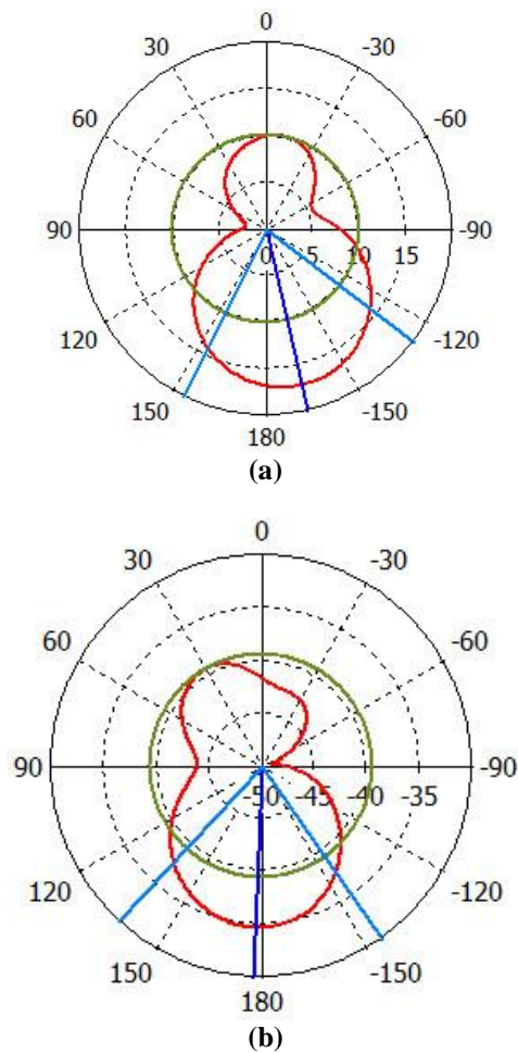
Fig. 11. Radiation patterns for the proposed reader antenna at 5.8GHz. (a) E-plane (b) H-plane.
