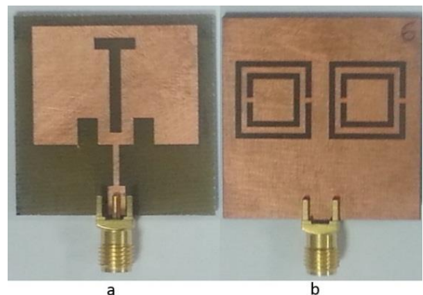
Fig. 13. Manufactured antenna.
