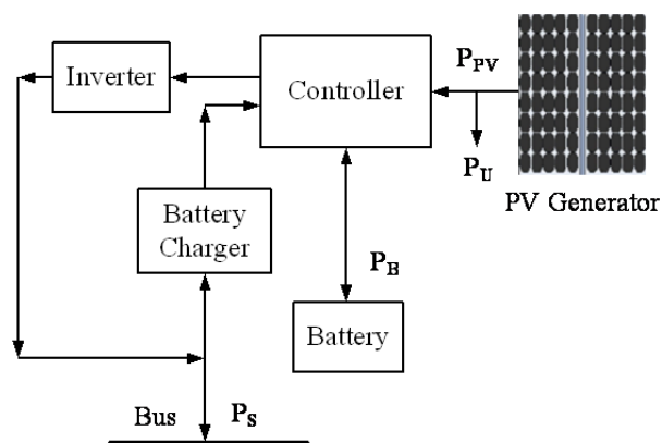
Fig. 1. Grid connected solar energy system with battery storage.
