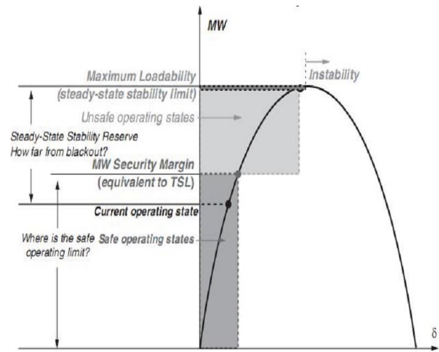
Fig. 1. Secure and Insecure operation states.
