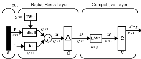
Fig.2. PNN Structure.
