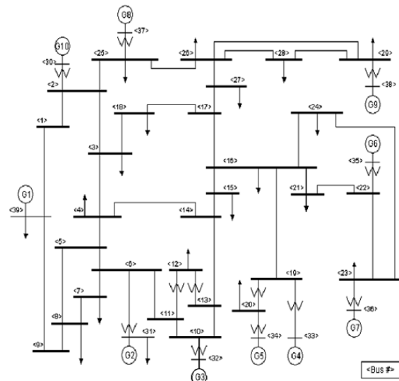
Fig. 3. IEEE 39 bus single line diagram.
